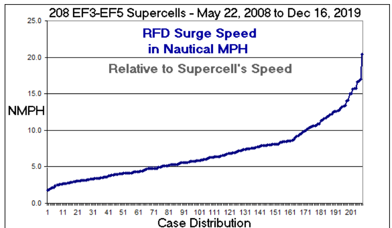
Figure 17. Sorted distribution of RFD surge storm relative speed for all 208 supercells. The average RFD surge storm relative speed ranged from just under two knots to just over 20 knots. The RFD's primary role during tornadogenesis is to move the RFD boundary toward the FFD boundary, in order to create an inflow channel. A fast storm relative speed is not necessary to accomplish this task.
