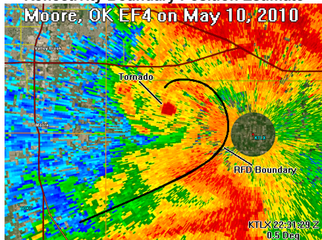
Figure 5. Estimate of RFD boundary position (black) using the reflectivity image for Moore, Oklahoma on May 10, 2010. For every RFD boundary estimate, both reflectivity and base velocity were used together, but one was chosen as primary.
