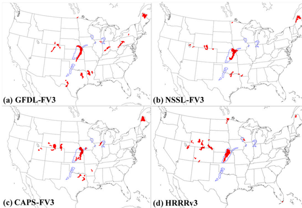
FIG. 7. Reflectivity objects greater than or equal to 30 dBZ at forecast hour 23 for (a) the GFDL-FV3, (b) the NSSL-FV3, (c) the CAPS-FV3, and (d) the HRRRv3 at 2300 UTC 2 May 2018. Model-simulated reflectivity objects are shown by the red filled contours, and observed reflectivity objects are shown by the blue contours.
