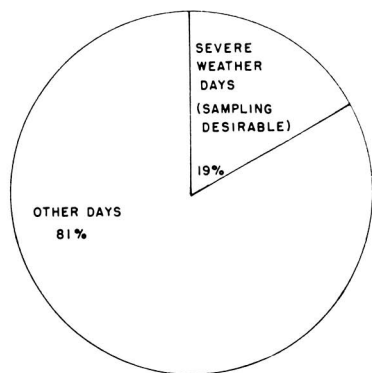
A. PERCENT OF TOTAL AVAILABLE TIME, (FEB. 1—MAY 31, 1959) THAT SYNOPTIC WEATHER PATTERN MADE SAMPLING DESIRABLE.
