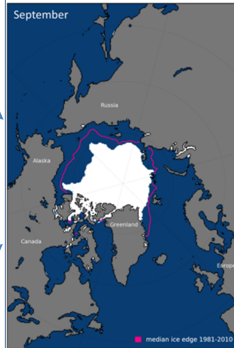
Sea Ice Extent September 2017 Summer minimum
