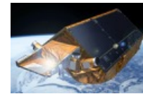
CryoSat-2 2012
