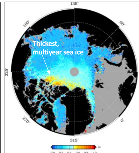
NASA ICESat-2
