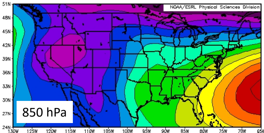
850mb Geopotential Height (m) Composite Mean 7/1/13 to 7/31/13 NCEP/NCAR Reanalysis
