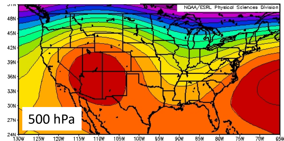
500mb Geopotential Height (m) Composite Mean 7/1/13 to 7/31/13 NCEP/NCAR Reanalysis
