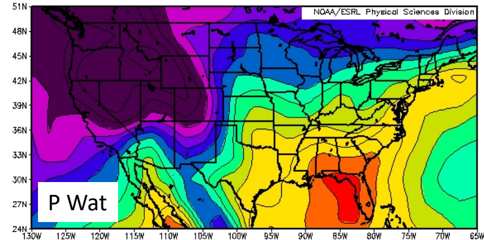
Columnar Precipitable Water \text{kg/m}^2 Composite Mean 7/1/13 to 7/31/13 NCEP/NCAR Reanalysis
