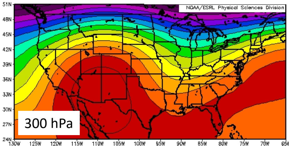
300mb Geopotential Height (m) Composite Mean 7/1/13 to 7/31/13 NCEP/NCAR Reanalysis
