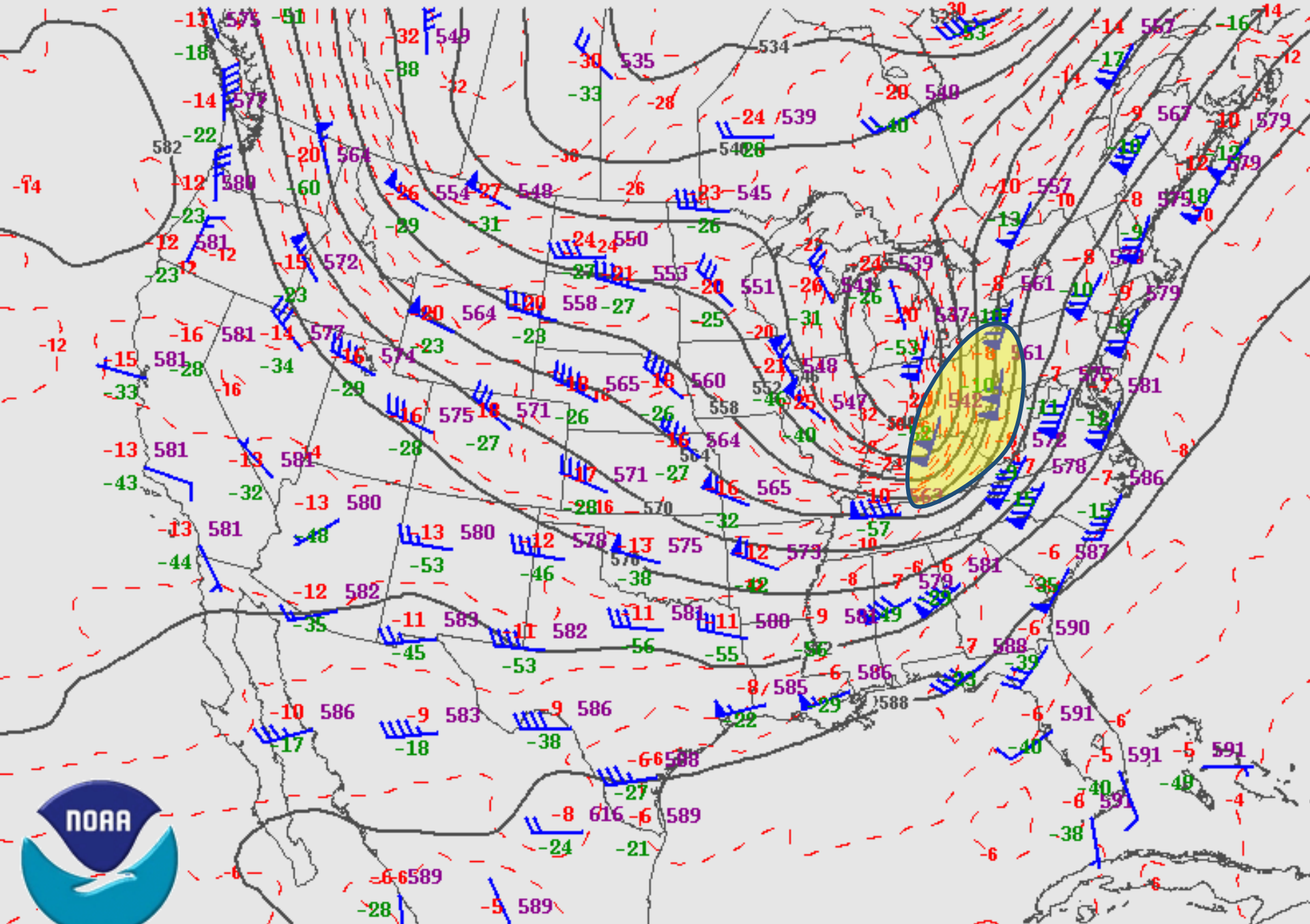
191101/0000 500 MB UA OBS, HGHTS, and TEMPS
