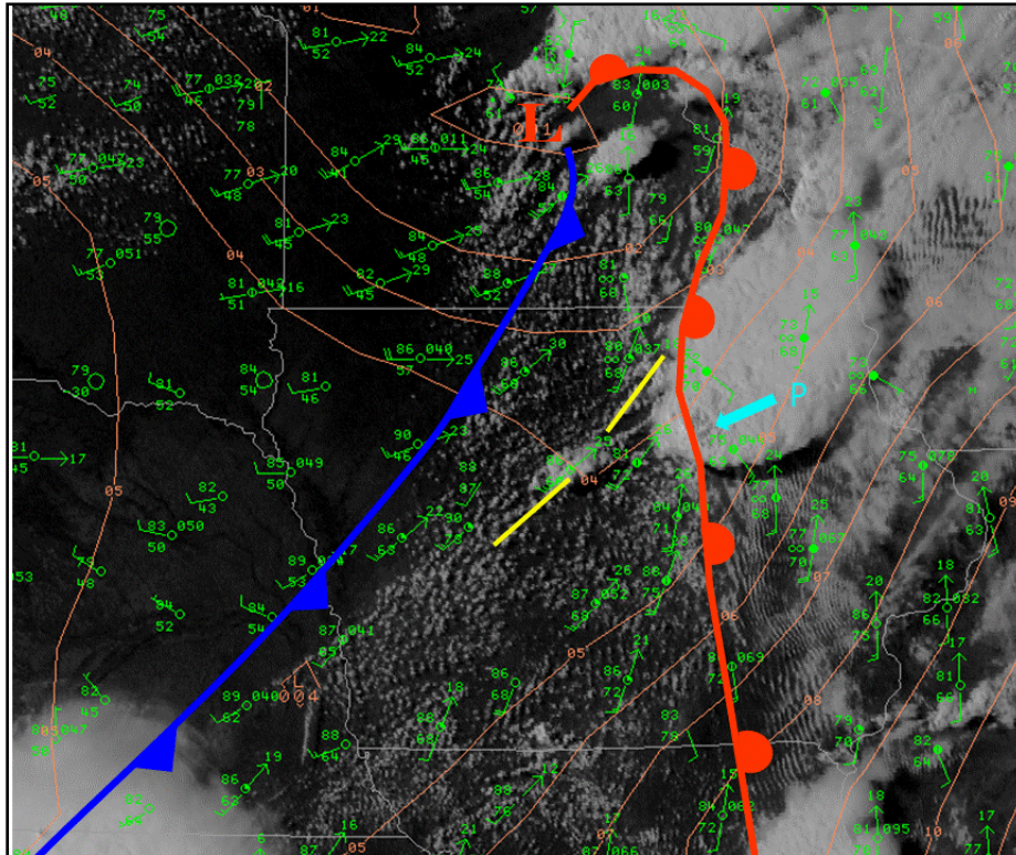
Fig. 5. MSLP, surface observations, surface analysis, and visible satellite imagery, 2200 UTC 25 May 2008 (cyan arrow indicates location of Parkersburg)
