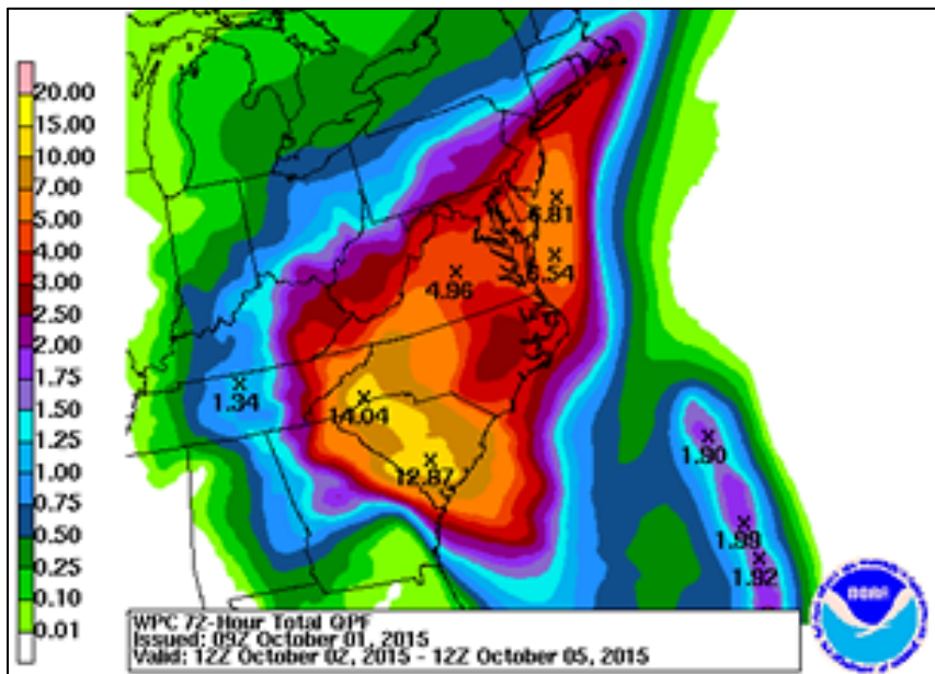
Figure 23: WPC 72-Hour QPF issued at 0900 UTC on October 1. Source: Weather Prediction Center
