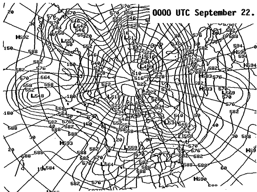
Fig. 1. 500 mb hemispheric initial height analysis
