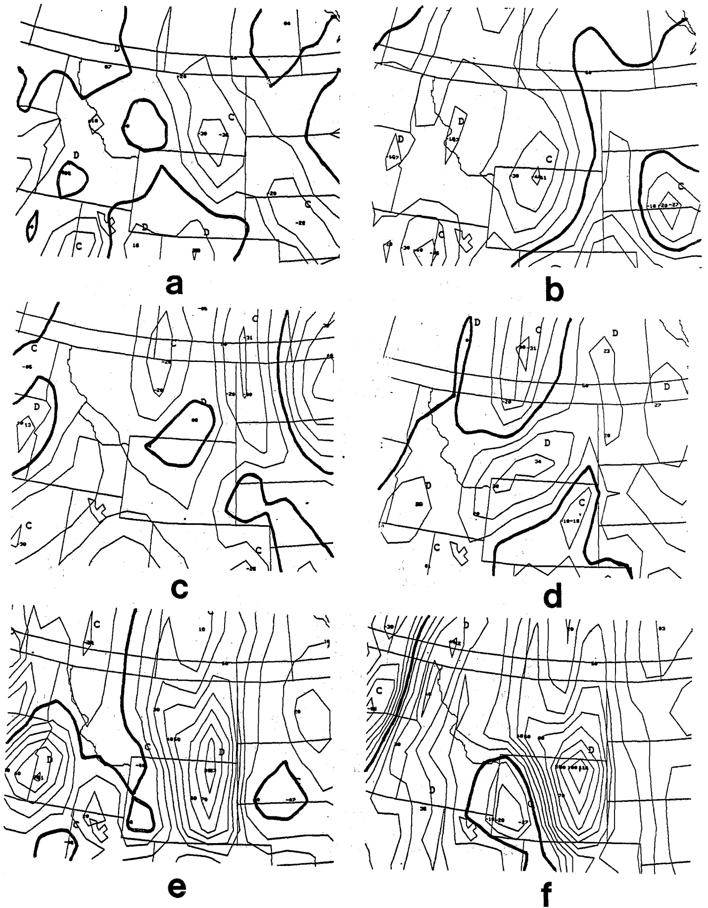
Fig. 14. Mesoanalysis of convergence at 0000 UTC September 25 at a) surface, b) 850 mb, c) 700 mb, d) 500 mb, e) 300 mb and f) 250 mb. Values based on 1.4^\circ latitude \times 1.2^\circ longitude grid with 2 smoothing passes. Negative values indicate convergence, units are 10^{-6} \text{ sec}^{-1} with a contour interval of 10. Heavy line is zero contour.
