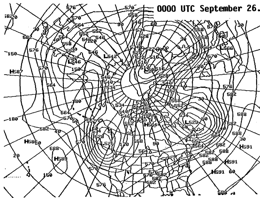
Fig. 2. MRF 96-hour forecast of 500 mb heights valid
