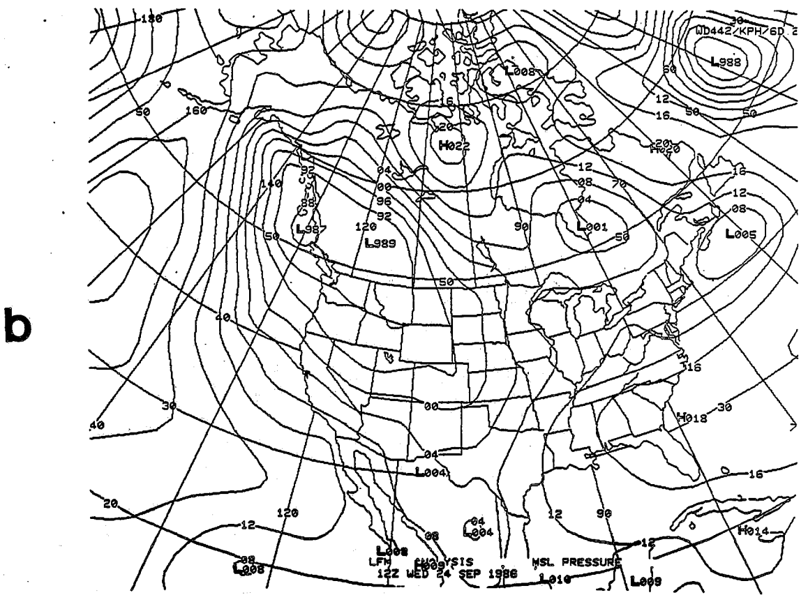
Fig. 6. LFM sea level pressure initial analyses for a) 0000 UTC September 24, b) 1200 UTC September 24, c) 0000 UTC September 25 and d) 1200 UTC September 25.
