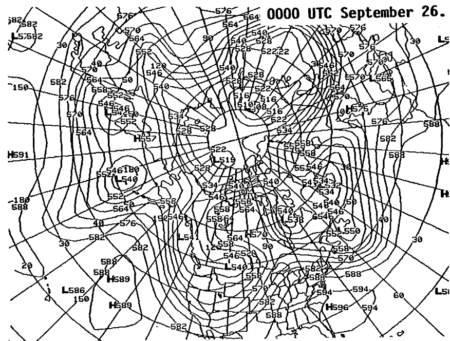
Fig. 3. 500 mb hemispheric initial height analysis
