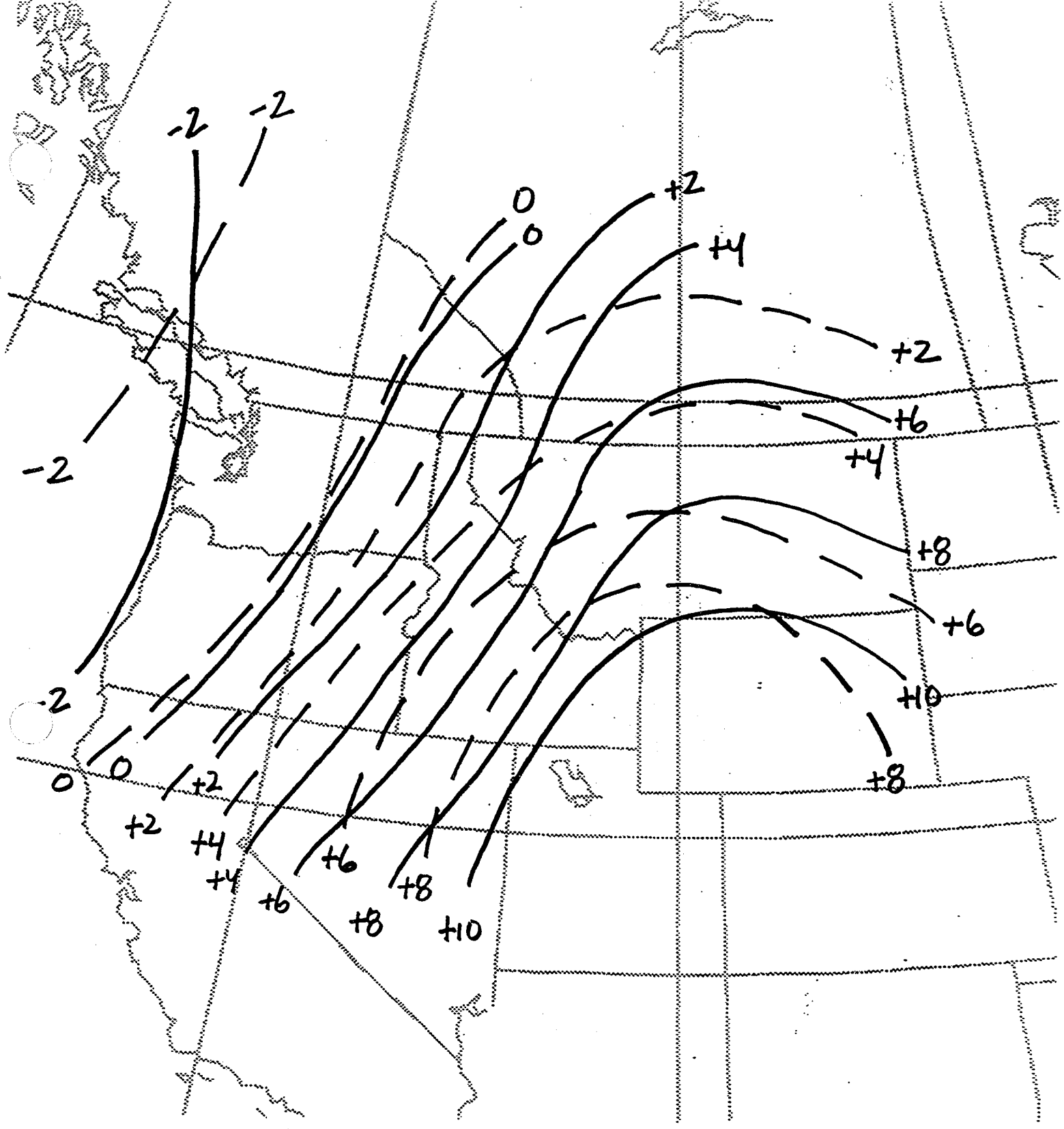
Figure 17: Average 700 mb temperatures in degrees Celsius at 1200 UTC (dashed) and 0000 UTC (solid) during Pattern B SSWEs in Idaho, Montana, and Wyoming.
