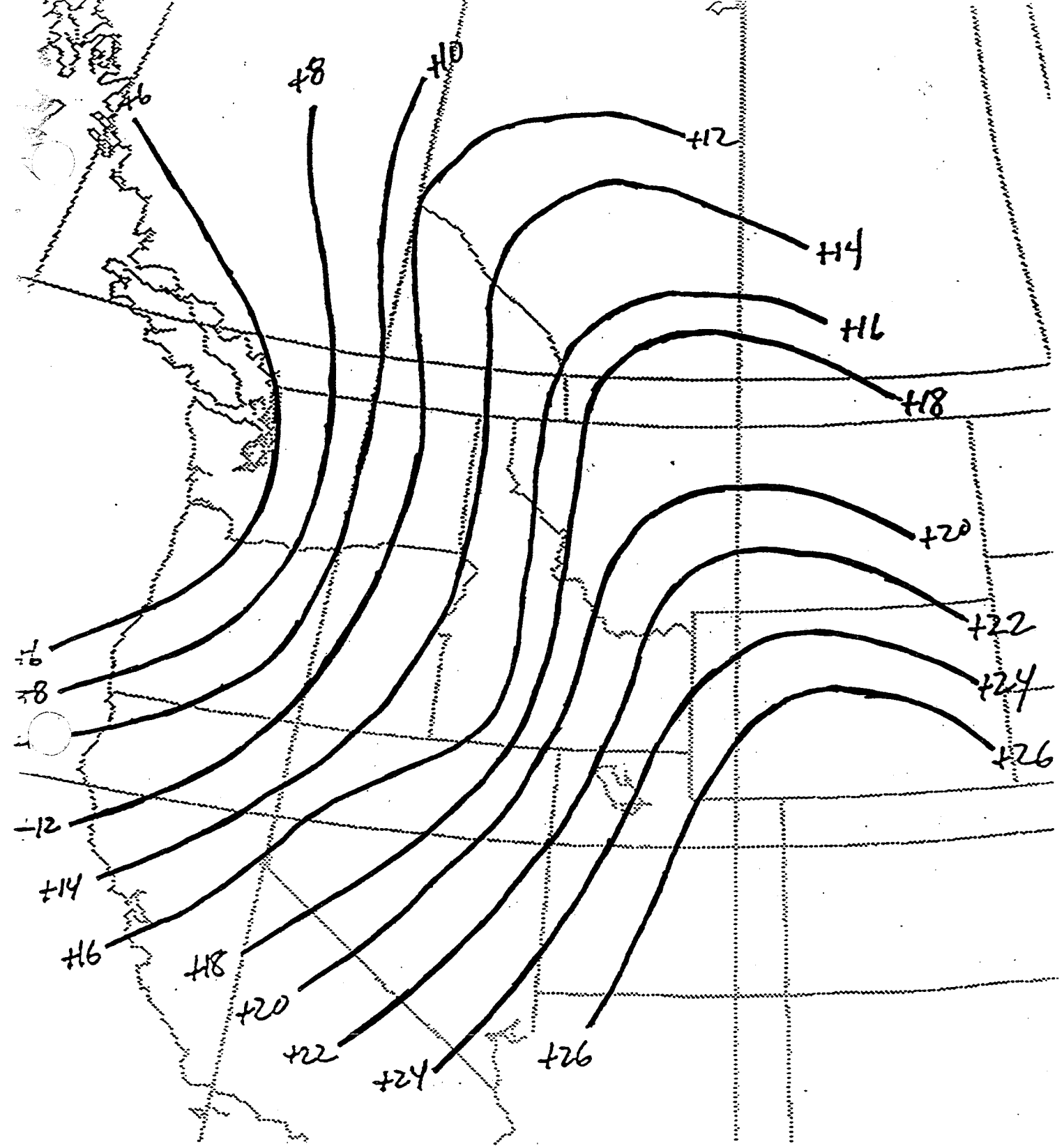
Figure 11: Average 850 mb temperatures in degrees Celsius at 0000 UTC during Pattern A SSWEs in Idaho, Montana, and Wyoming.
