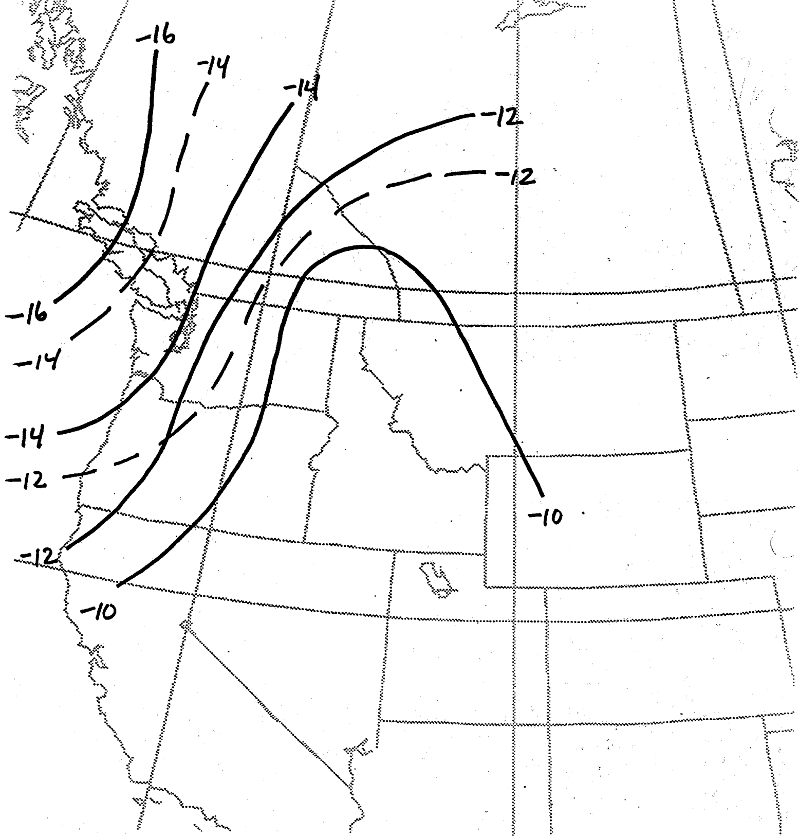
Figure 22: Average 500 mb temperatures in degrees Celsius at 1200 UTC (dashed) and 0000 UTC (solid) during Pattern A SSWEs in Washington and Oregon.
