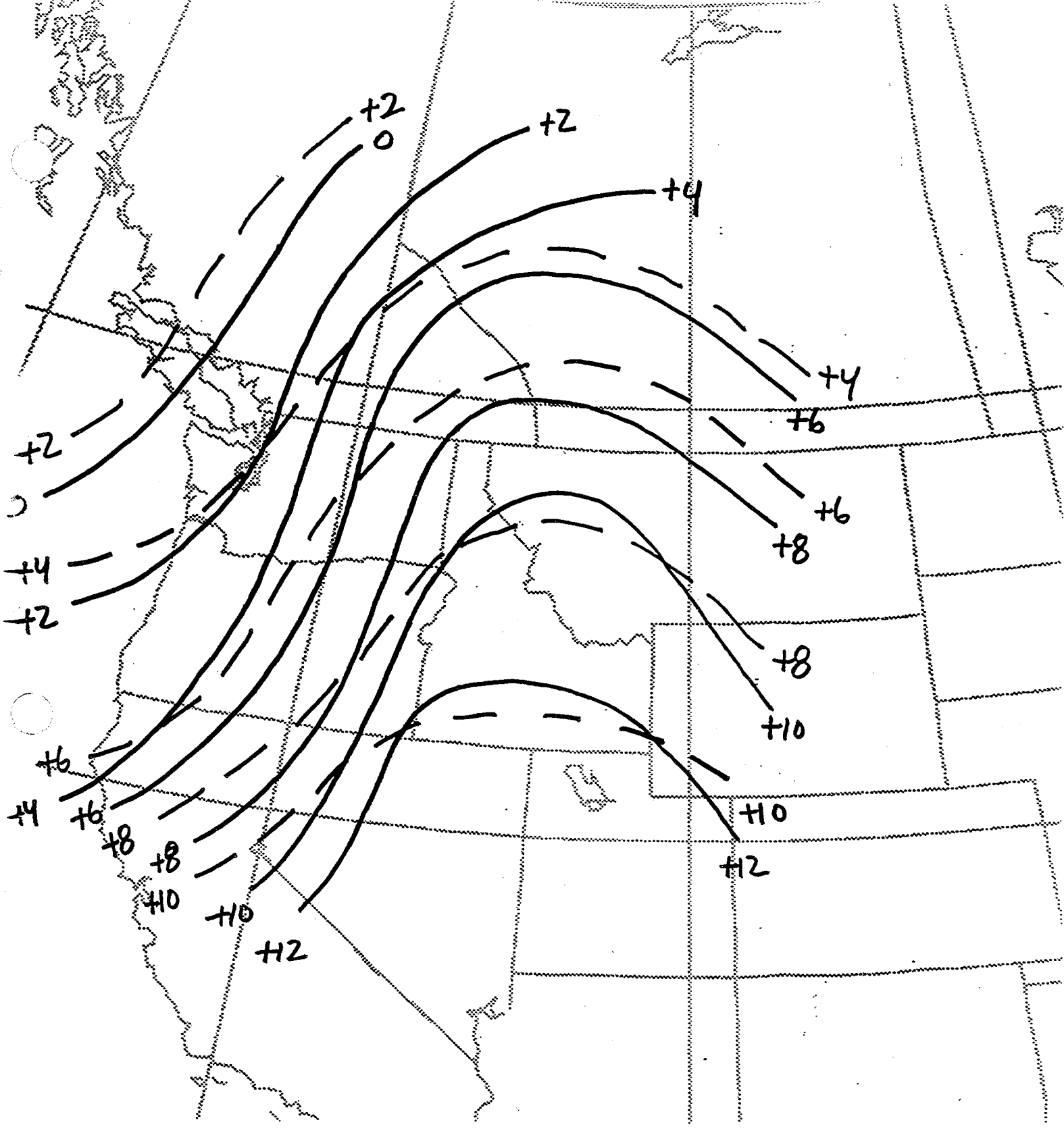
Figure 23: Average 700 mb temperatures in degrees Celsius at 1200 UTC (dashed) and 0000 UTC (solid) during Pattern A SSWEs in Washington and Oregon.
