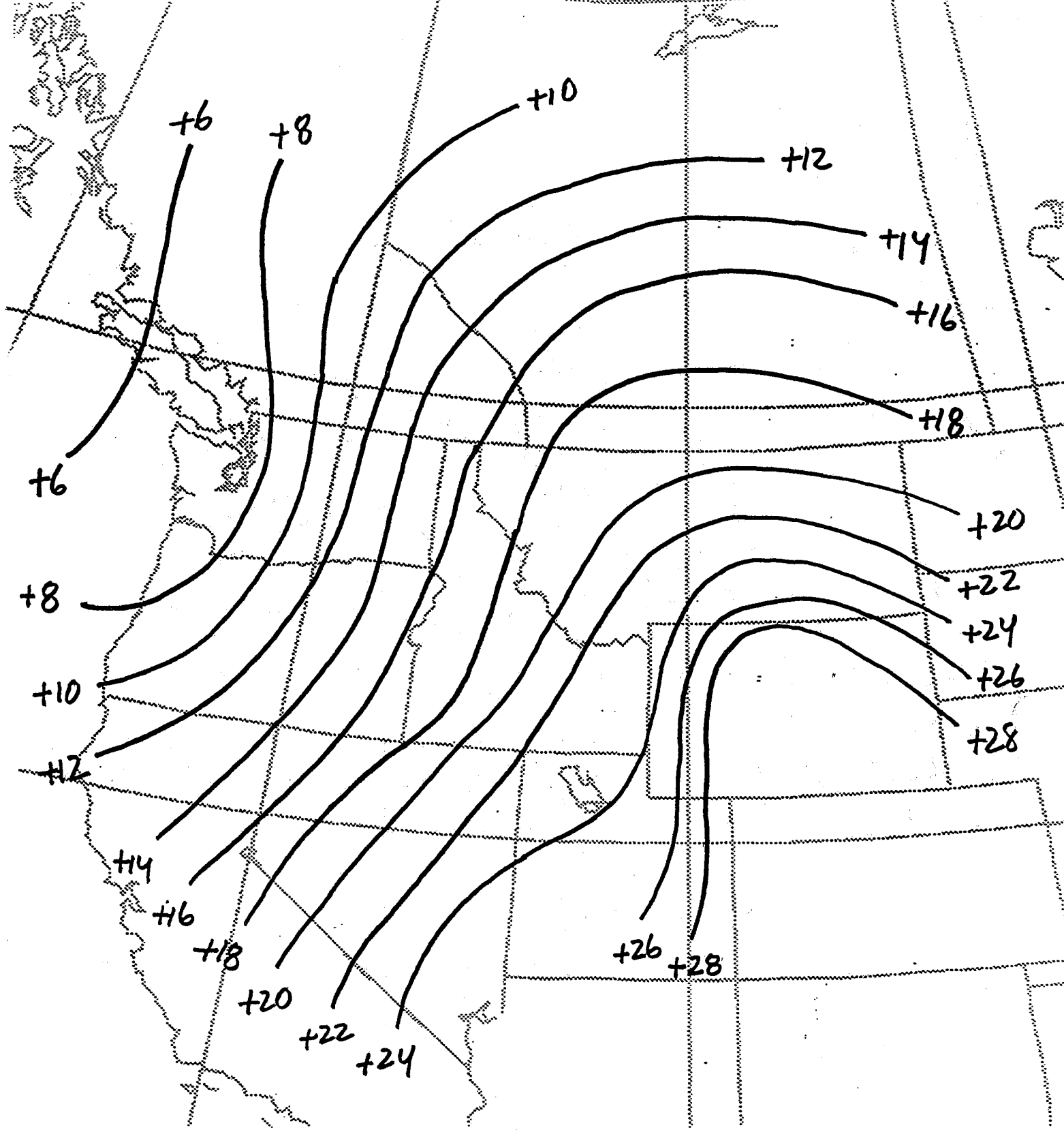
Figure 18: Average 850 mb temperatures in degrees Celsius at 0000 UTC during Pattern B SSWEs in Idaho, Montana, and Wyoming.
