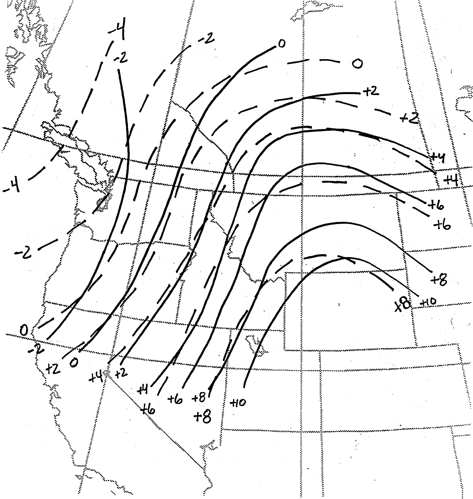
Figure 12: Average 700 mb temperatures in degrees Celsius at 1200 UTC (dashed) and 0000 UTC (solid) during Pattern A SSWEs in Idaho, Montana, and Wyoming.
