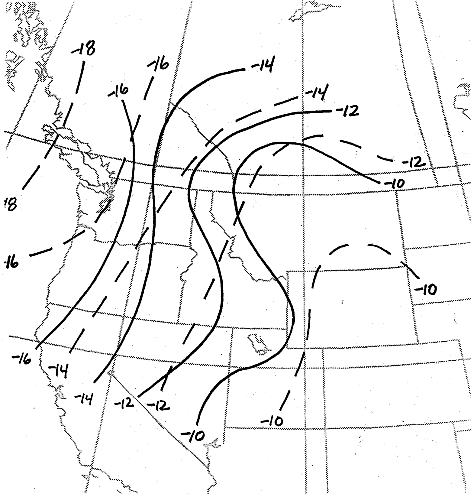
Figure 16: Average 500 mb temperatures in degrees Celsius at 1200 UTC (dashed) and 0000 UTC (solid) during Pattern B SSWEs in Idaho, Montana, and Wyoming.
