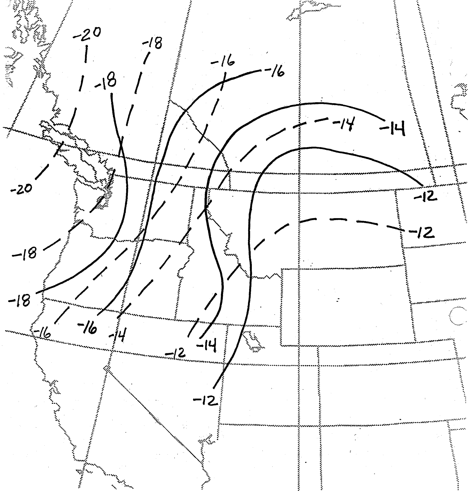
Figure 10: Average 500 mb temperatures in degrees Celsius at 1200 UTC (dashed) and 0000 UTC (solid) during Pattern A SSWEs in Idaho, Montana, and Wyoming.
