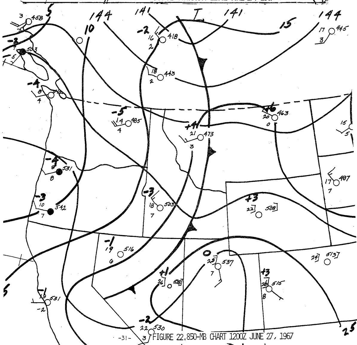
FIGURE 21. 500-MB VORTICITY 1200Z JUNE 27, 1967
