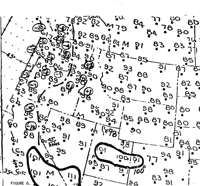
FIGURE 6. MAXIMUM TEMPERATURE CHART FOR PERIOD ENDING 0000Z JUNE 23, 1971 (i.e., TEMPERATURES ON JUNE 22). CIRCLED PLUS AND MINUS FIGURES ARE 24-HOUR TEMPERATURE CHANGES.
