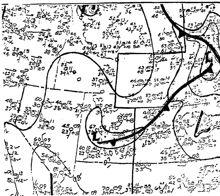
FIGURE 7. NMC ANALYSIS 1200Z JUNE 24, 1971. HEAVY FRONTAL LINES ARE NMC ORIGINAL ANALYSIS.
