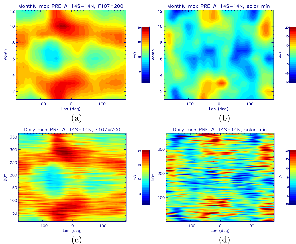
Figure 11. (a,b) Monthly averaged values of maximum preverval enhancement (PRE) between 14°S and 14°N from WACCM-X simulations under solar maximum and solar minimum conditions, respectively. (c, d) Similar to Figures 11a and 11b but daily values of PRE.
