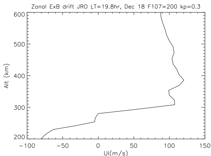
Figure 10. Vertical profile of zonal E \times B drift at 12.3^{\circ}\text{S}/77.5^{\circ}\text{W} and 1948 LT on 18 December of the simulation under solar maximum conditions.
